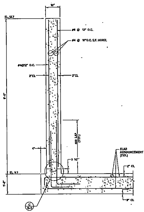
TYPICAL WALL SECTION 1 SCALE: 1" = 1'-0"
